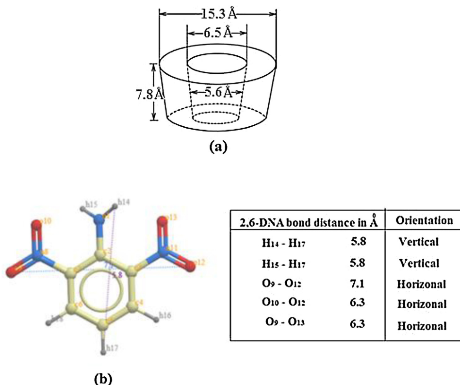
Scheme 4. Schematic representation of semi empirical bond distance of (a) \beta -CD, (b) 2,6-DNA. (For interpretation of the references to color in this scheme legend, the reader is referred to the web version of this article.)
