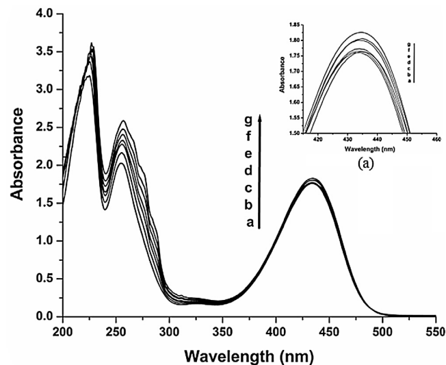
Fig. 2. Absorption spectra of 2,6-DNA (conc. 2 \times 10^{-4} M) in pH ~ 7 solutions at different \beta -CD ((a)–(g) conc. 0 – 12 \times 10^{-3} M). Inset (a) magnified view of \beta -CD effect in pH ~ 7 solution at 432 nm.
