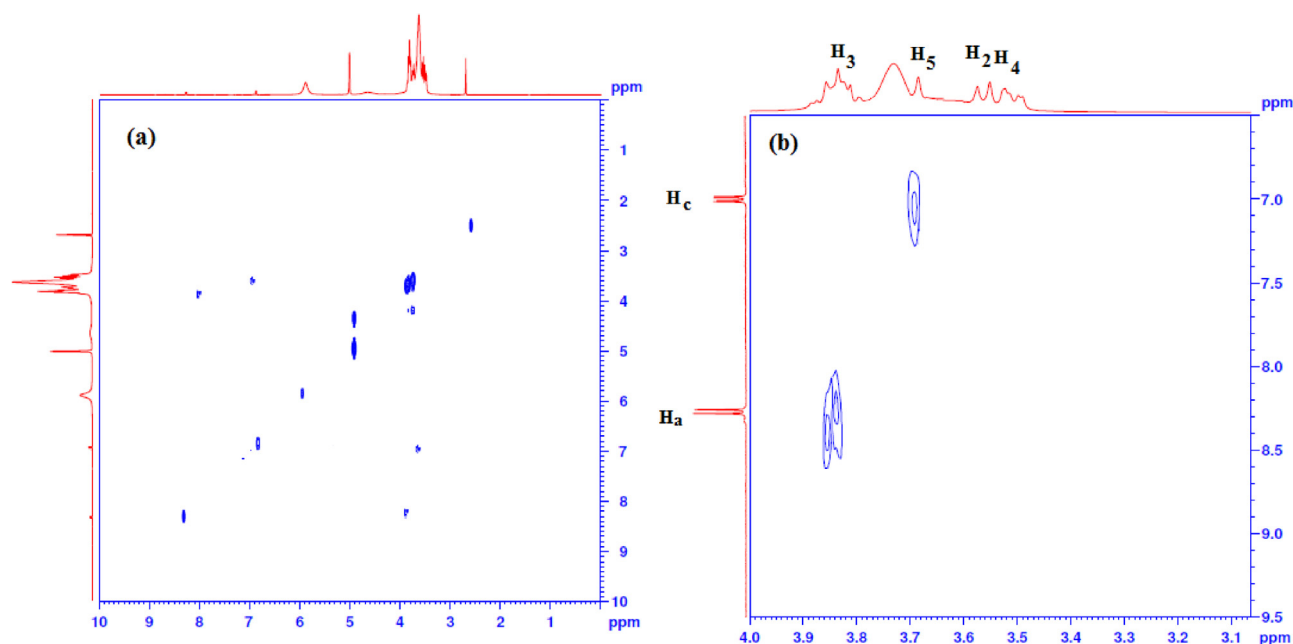
Fig. 5. The 2D ^1\text{H} NMR (ROESY) spectra of inclusion complex of (a) 2,6-DNA: \beta -CD, (b) partial counter plot of 2,6-DNA: \beta -CD in \text{DMSO-d}_6 at 300 K.
