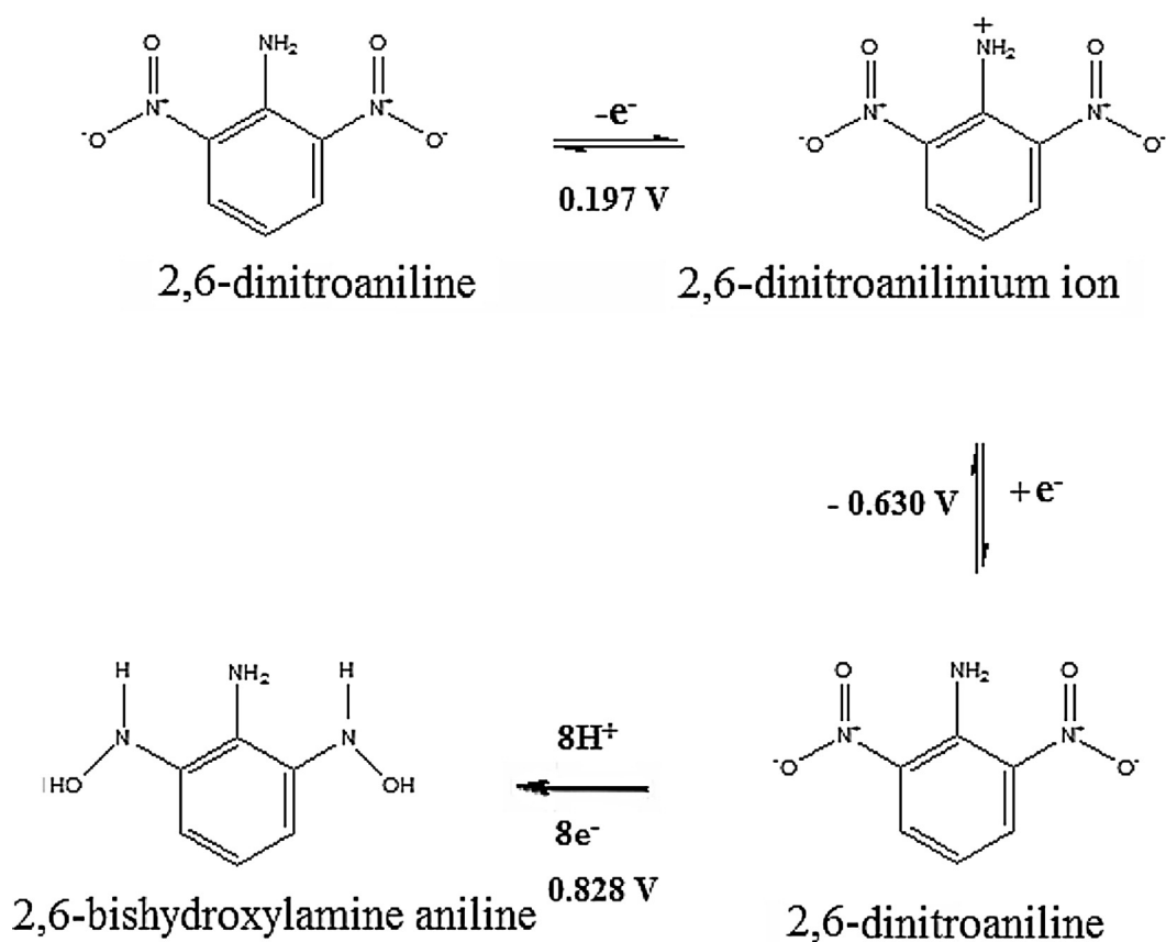
Scheme 6. Reaction mechanism of 2,6-DNA in pH ~ 7 buffer solution at glassy carbon electrode.
