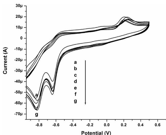
Fig. 3. Cyclic voltammograms for 2,6-DNA: \beta -CD in pH \sim 7 buffer solution, scan rate 100 mV/s, 2,6-DNA (conc. 2 \times 10^{-4} M) and \beta -CD ((a)–(g) conc. 0 – 12 \times 10^{-3} M).
