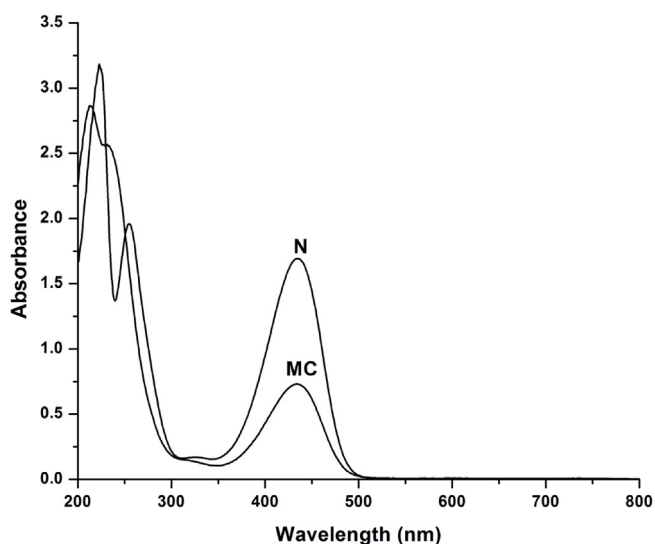
Fig. 1. Absorption spectra of different prototropic species of 2,6-DNA at 303 K; concentration 2 \times 10^{-4} M (MC) monocation and (N) neutral.
