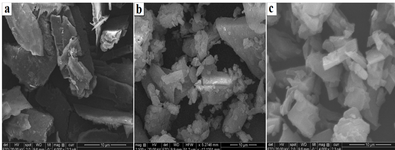
Fig. 8. Scanning electron microscope photographs (Pt. coated) of (a) 2,6-DNA (b) \beta -CD and (c) solid inclusion complex of 2,6-DNA: \beta -CD.
