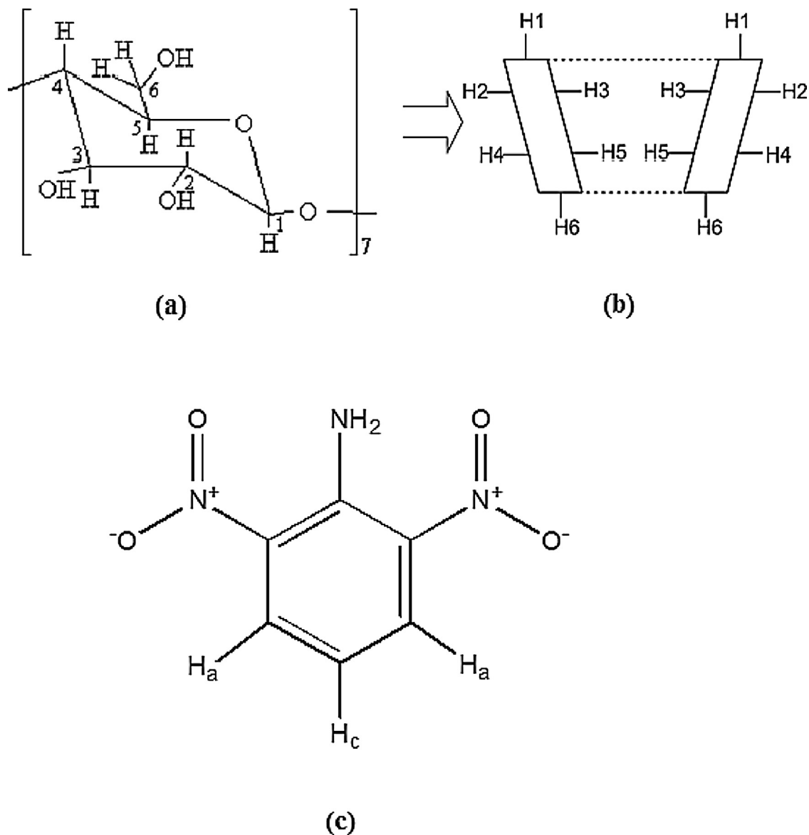
Scheme 7. (a) The stereo-configuration of \beta -CD, (b) truncated-cone shape of \beta -CD and (c) 2,6-DNA.
