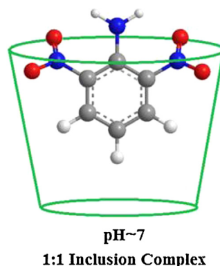
Scheme 3. The proposed structure of inclusion complex of (a) 2,6-DNA with \beta -CD. The oxygen atoms are shown as red, nitrogen as blue and carbon as gray color, hydrogen atoms are white.
