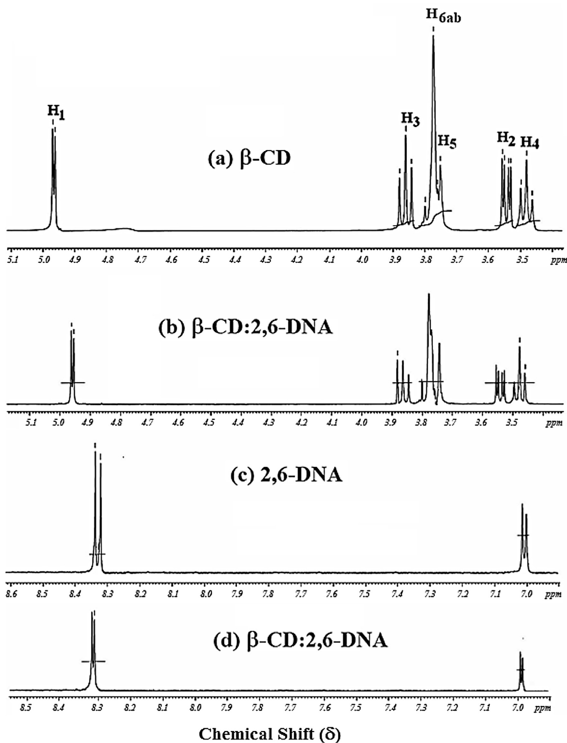
Fig. 4. ^1\text{H} NMR spectra of (a) \beta -CD, (b) the solid complex (chemical shift with respect to \beta -CD); (c) 2,6-DNA, (d) the solid complex (chemical shift with respect to 2,6-DNA).
