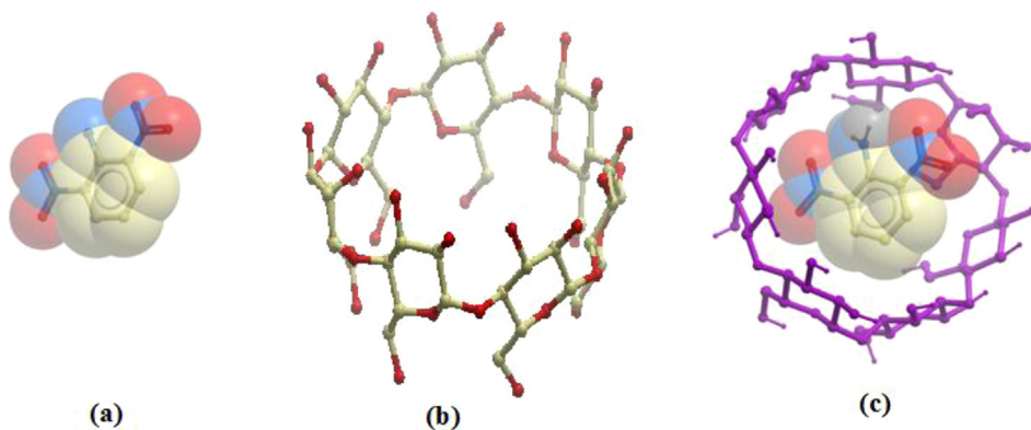
Scheme 5. Ball and stick representation of (a) 2,6-DNA (b) \beta -CD (c) 2,6-DNA: \beta -CD inclusion complex; the oxygen atoms are shown as red ball, nitrogen as blue and carbon as gray balls; hydrogen atoms are white balls. (For interpretation of the references to color in this scheme legend, the reader is referred to the web version of this article.)
