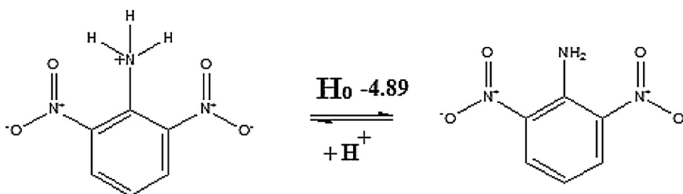
Scheme 2. Prototropic equilibria of 2,6-DNA in aqueous medium.
