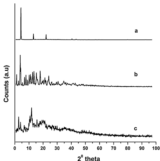
Fig. 7. Powder X Ray diffraction spectra of (a) 2,6-DNA, (b) \beta -CD and (c) solid inclusion complex of 2,6-DNA: \beta -CD.
