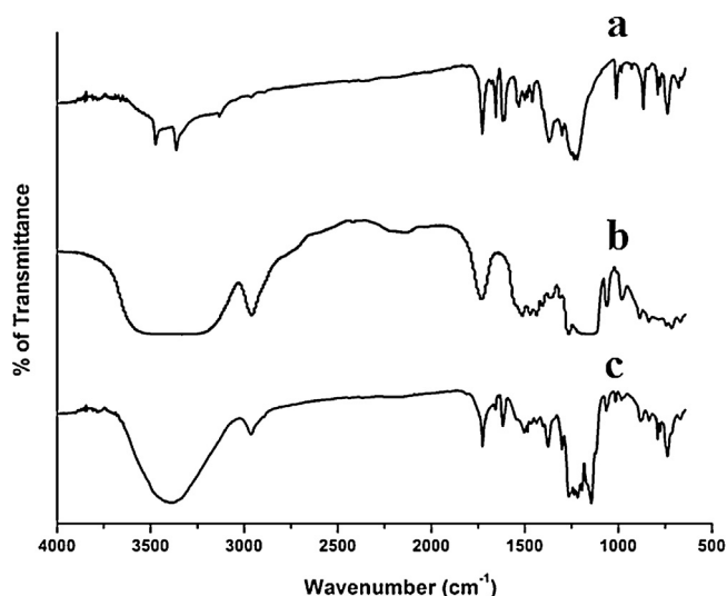
Fig. 6. FT-IR Spectra of (a) 2,6-DNA, (b) \beta -CD and (c) solid inclusion complex of 2,6-DNA: \beta -CD complex in KBr.
